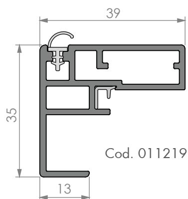
PROFILO MANIGLIA Handle profile
