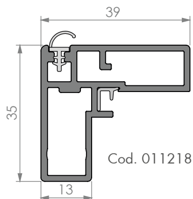
PROFILO CERNIERA Hinge profile
