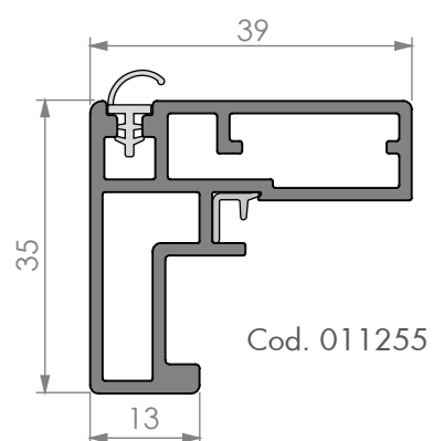
PROFILO MANIGLIA Handle profile
